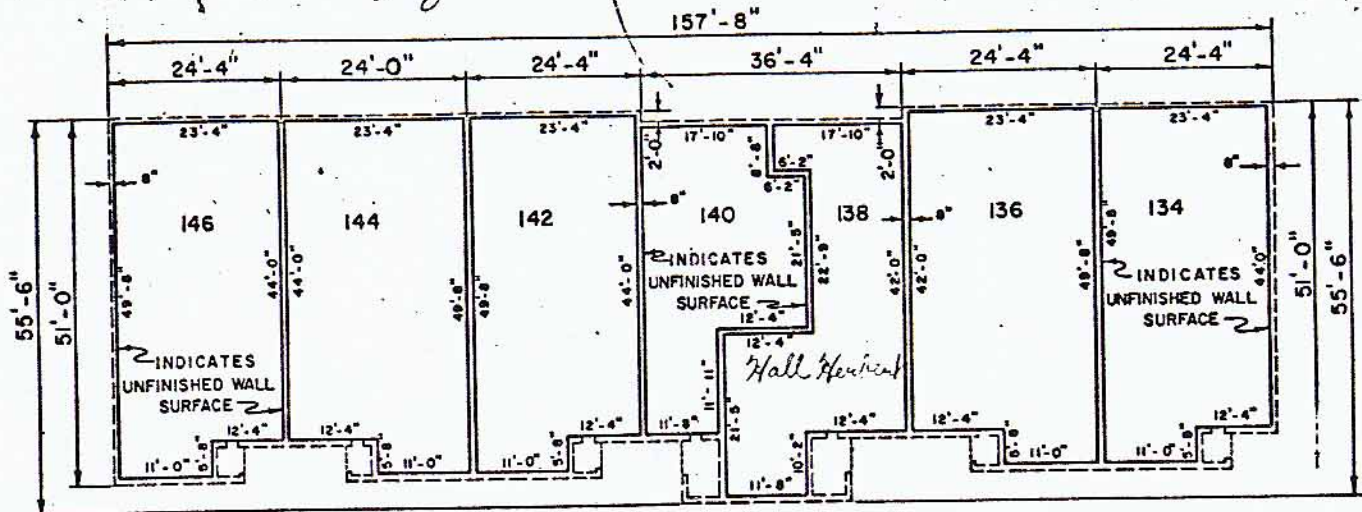
FLOOR PLAN BUILDING "4"
